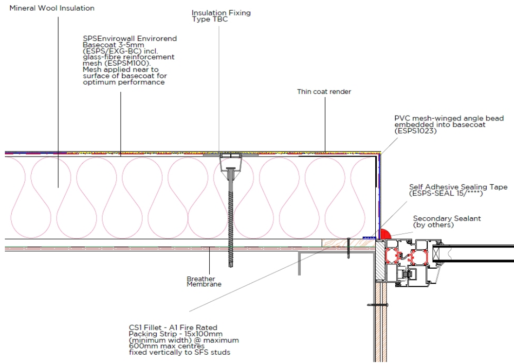
Figure 4 - Window reveal detail
