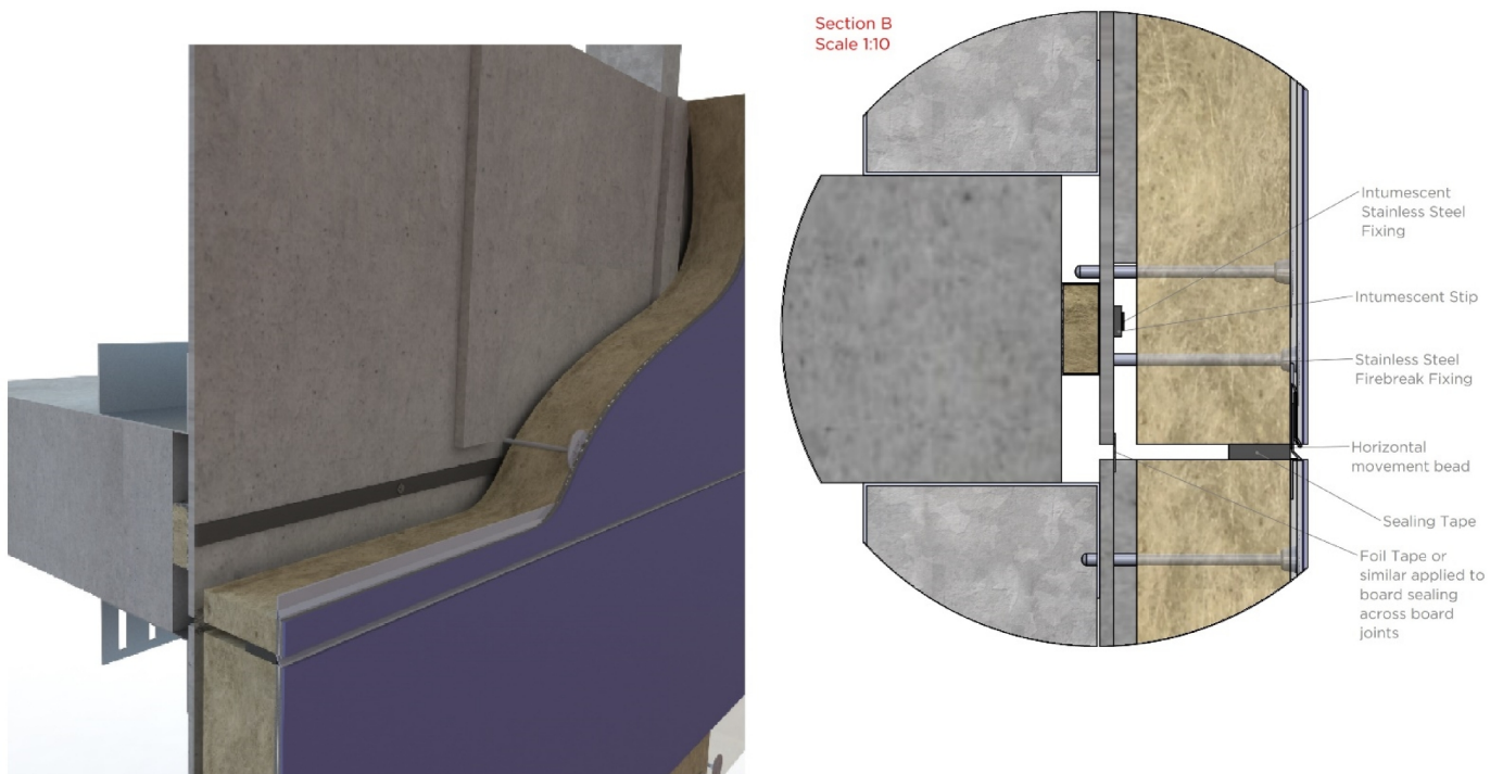
Figure 5 - Horizontal fire barrier detail
