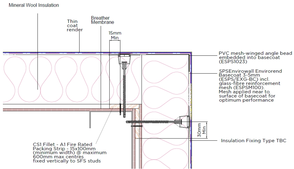
Figure 2 - External corner detail
