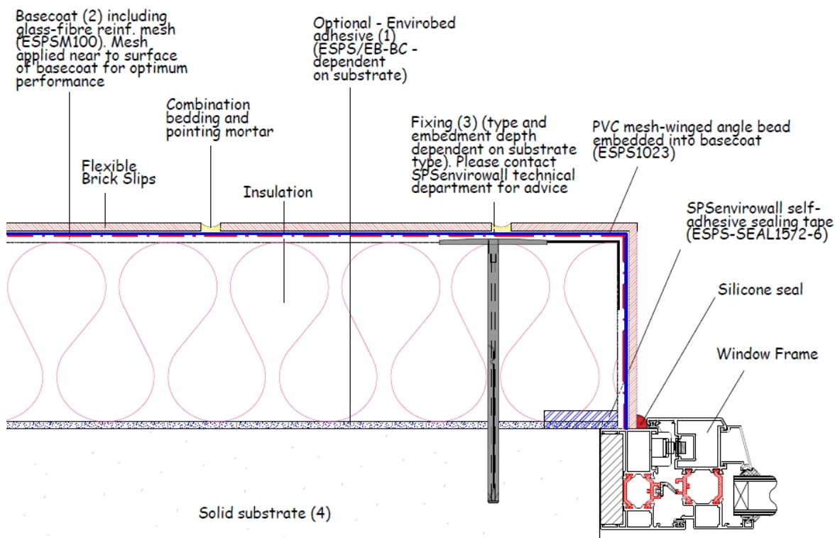
Figure 4 - Window reveal detail
