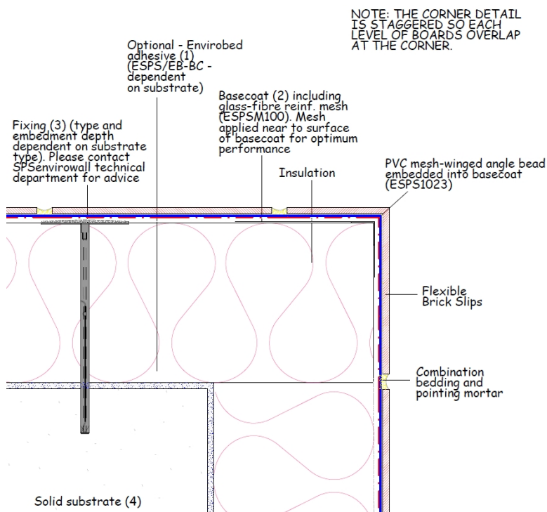
Figure 2 - External corner detail
