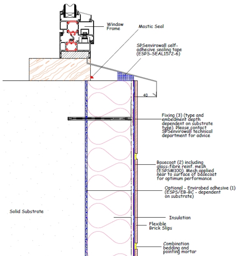
Figure 7 - Window cill detail
