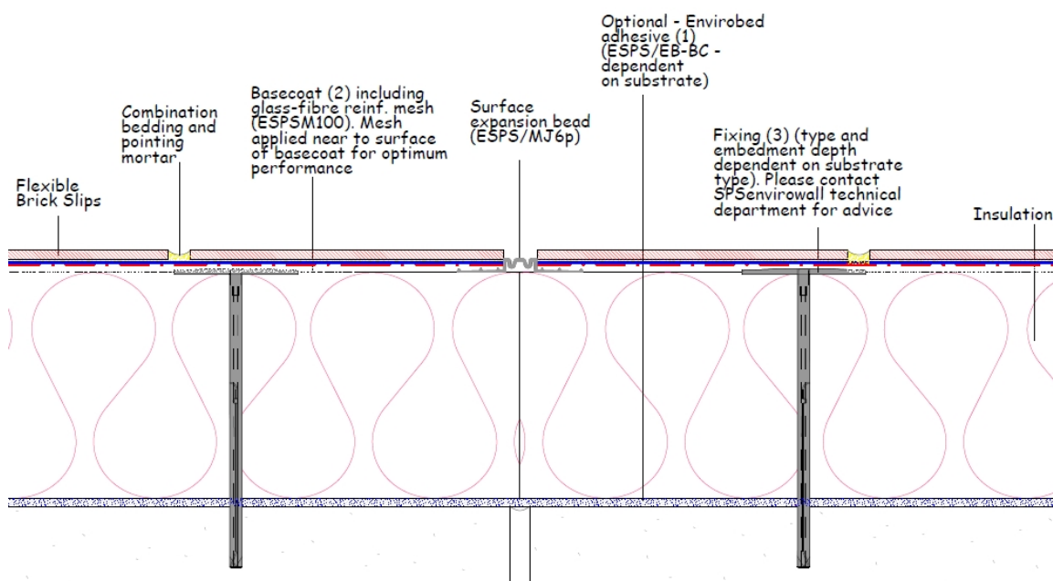
Figure 6 - Surface expansion bead
