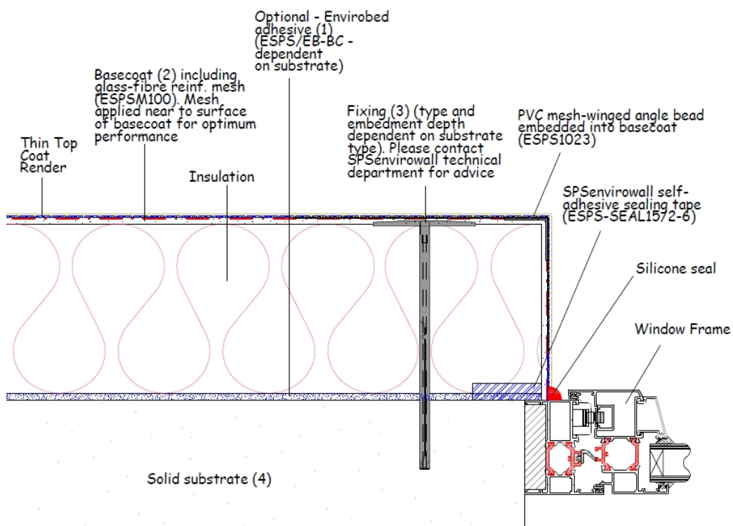
Figure 4 - Window reveal detail
