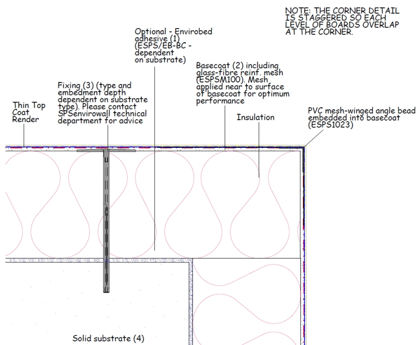
Figure 2 - External corner detail
