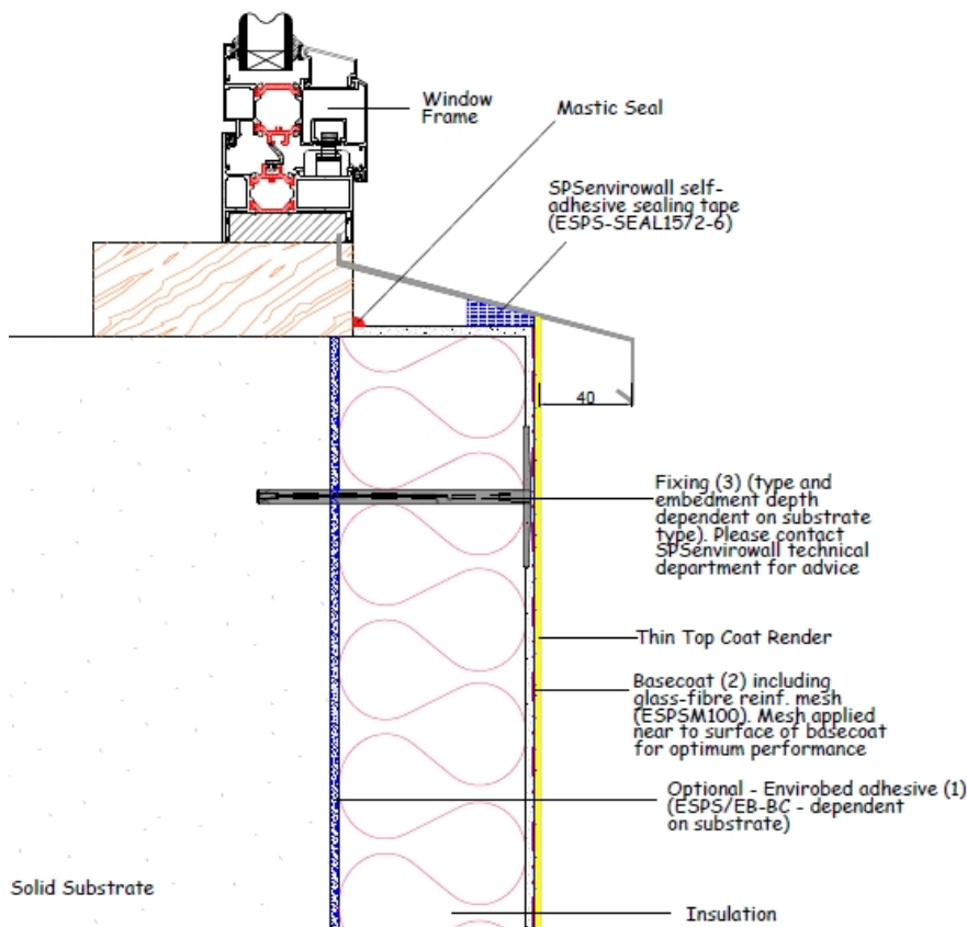
Figure 7 - Window cill detail
