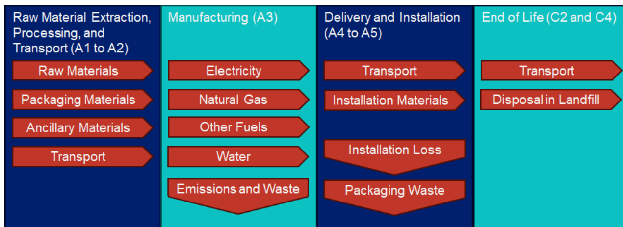
Figure 1-1: Simplified process flow diagram for 1/2" DensGlass® Sheathing
