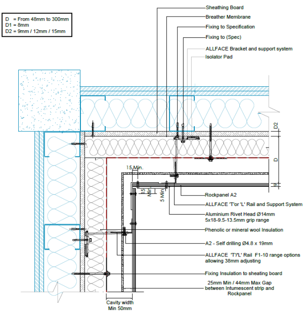
Diagram 11 - Typical internal corner fixed detail
