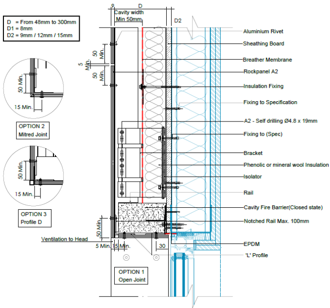
Diagram 9 - Typical window head detail
