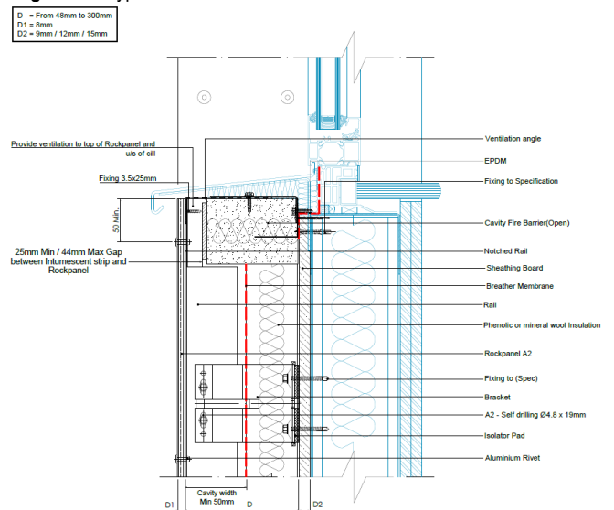
Diagram 8 - Typical window cill detail
