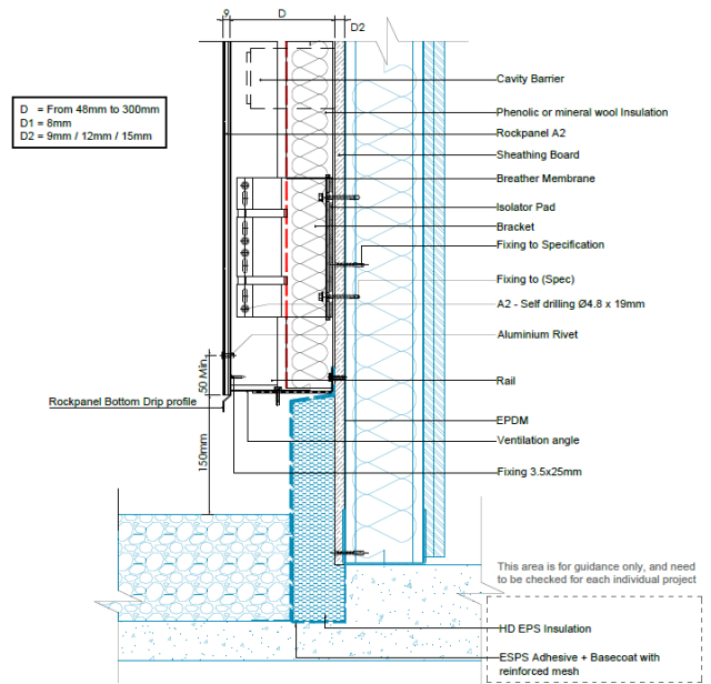
Diagram 10 - Typical base detail
