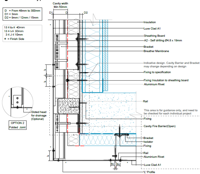
Diagram 13 - Typical soffit detail
