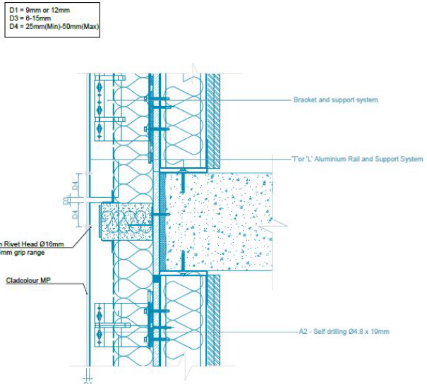
Diagram 3 - Typical installation detail of the Product on LGSF
