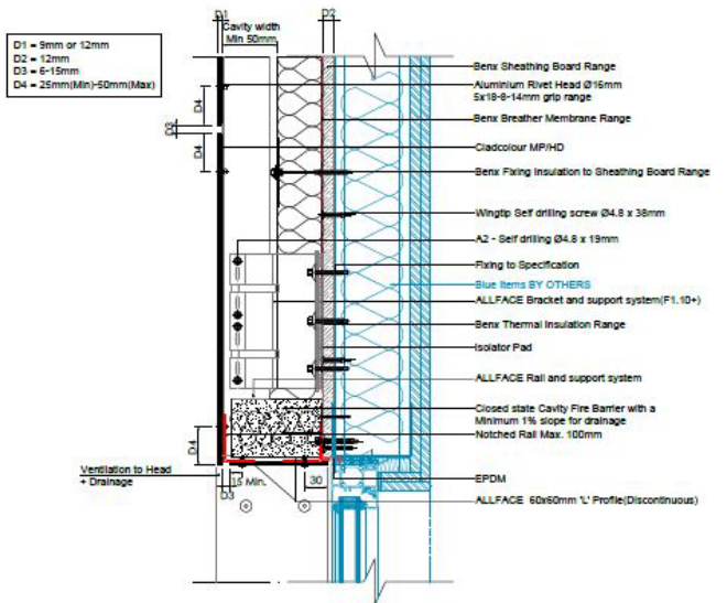
Diagram 8 - Typical window head detail
