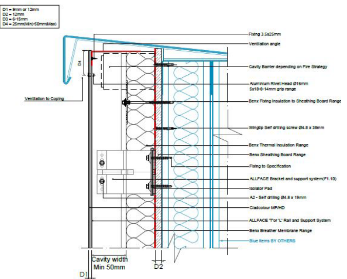
Diagram 10 - Typical coping detail
