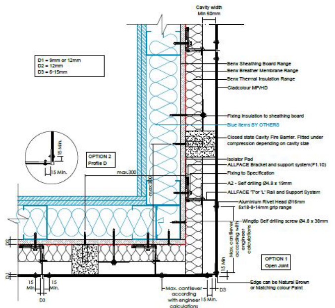
Diagram 12 - Typical external corner fixed detail
