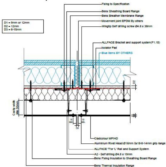
Diagram 13 - Movement joint vertical detail
