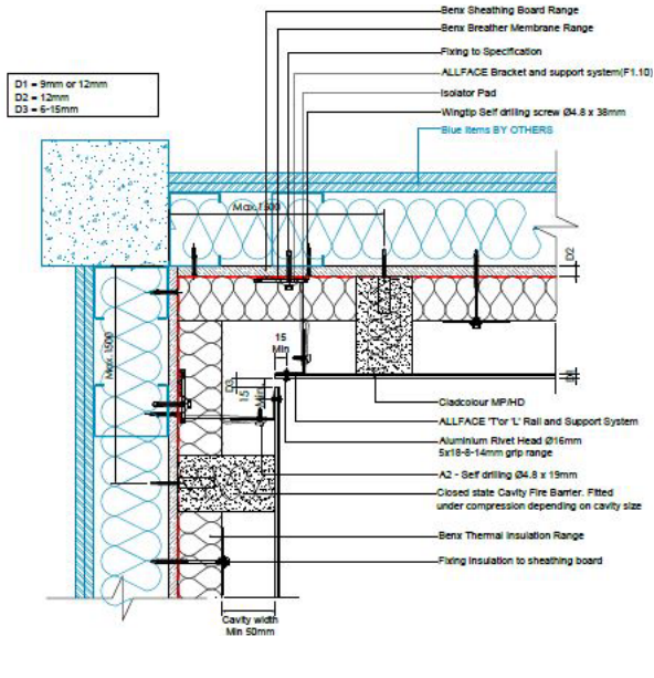
Diagram 11 - Typical internal corner cantilever detail
