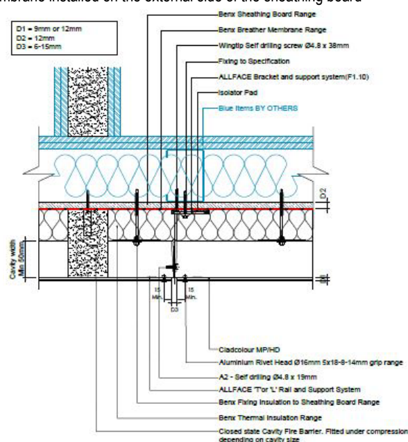
Diagram 4 - Plan view - typical construction detail of the System, breather membrane installed on the external side of the sheathing board
