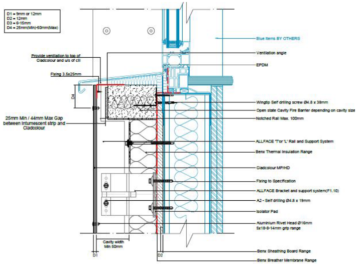
Diagram 7 - Typical window cill detail
