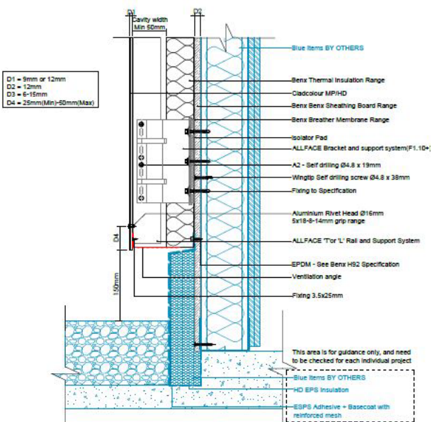
Diagram 9 - Typical base detail
