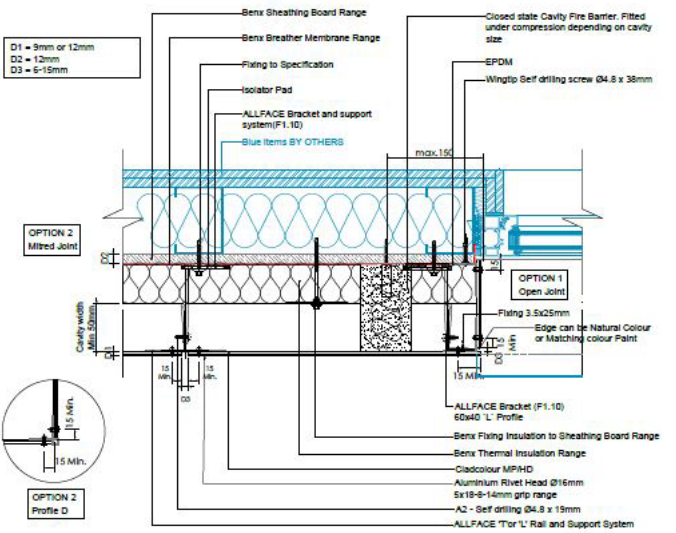
Diagram 8 - Typical window head detail
