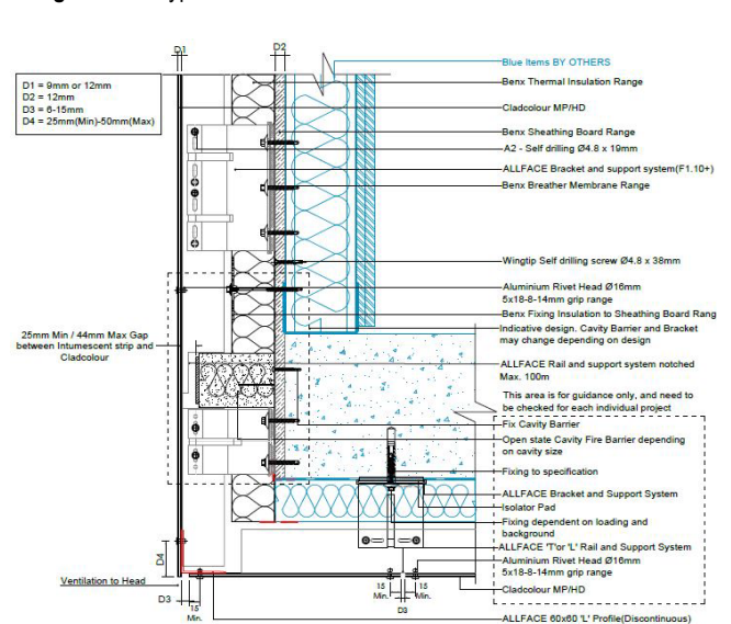
Diagram 14 - Typical soffit detail
