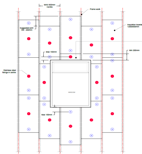
Diagram 3 - Typical insulation fixing pattern
