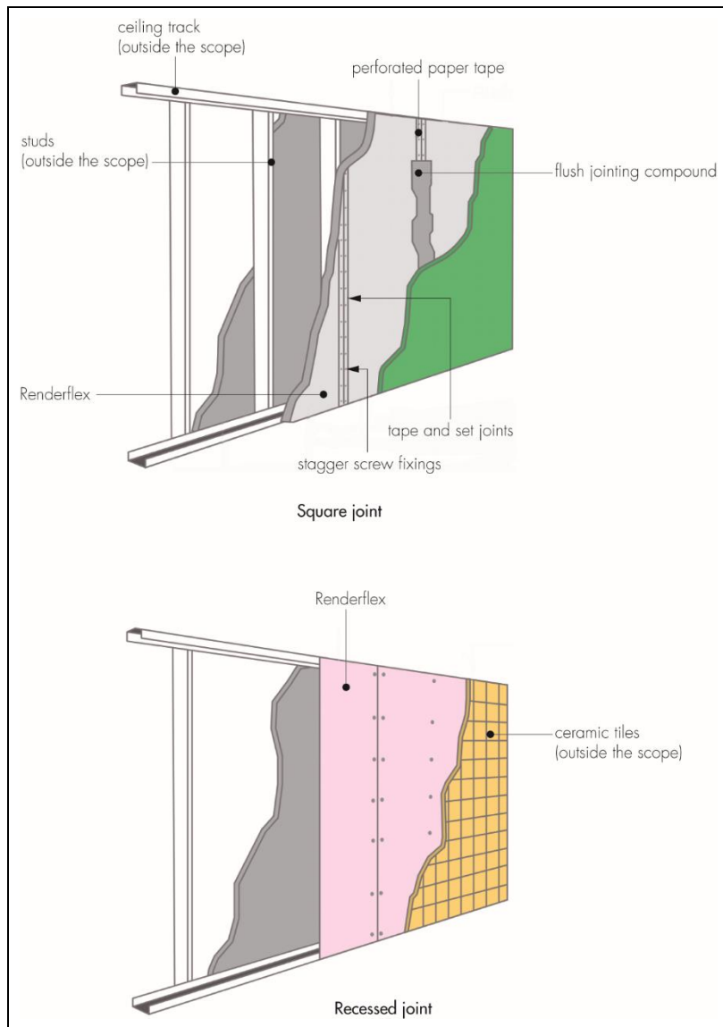
Figure 1 Typical installation
