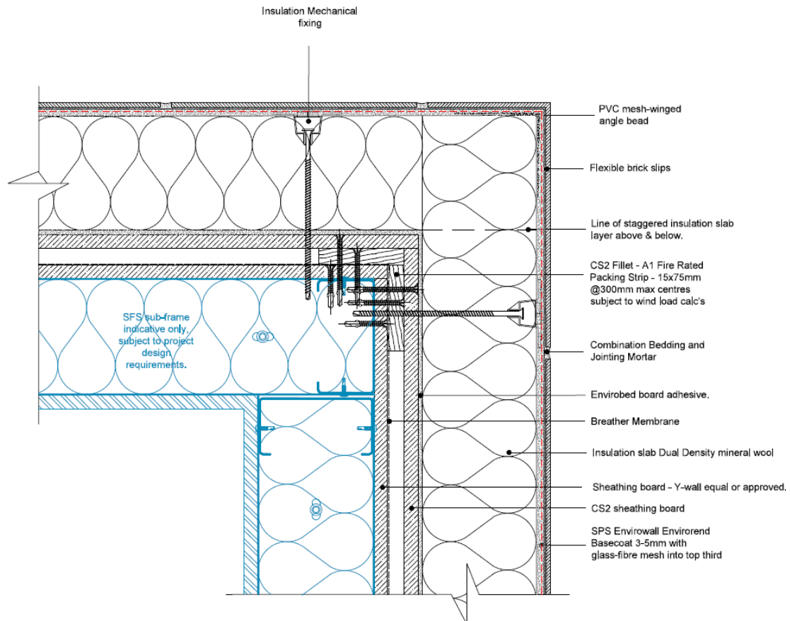
Diagram 2 - External corner detail
