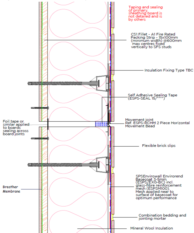
Diagram 8 - Window cill detail
