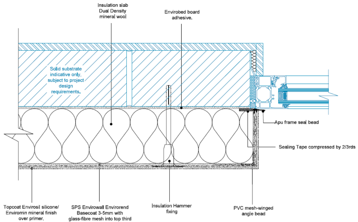
Diagram 3 - Window reveal detail
