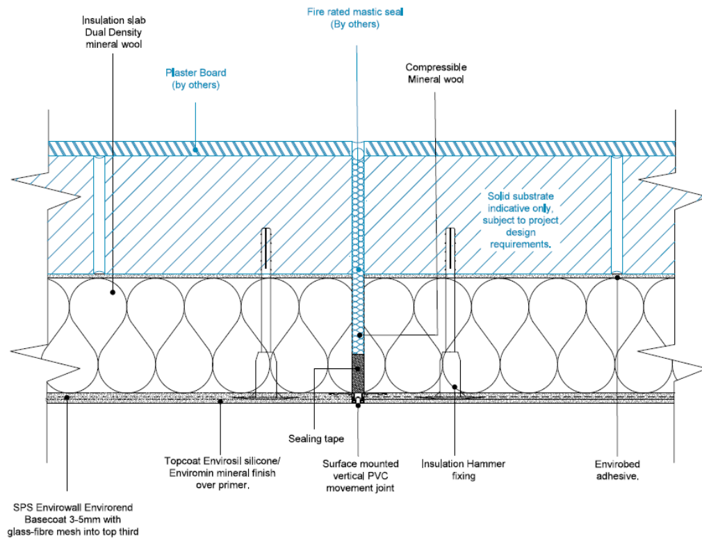
Diagram 5 - Surface expansion bead
