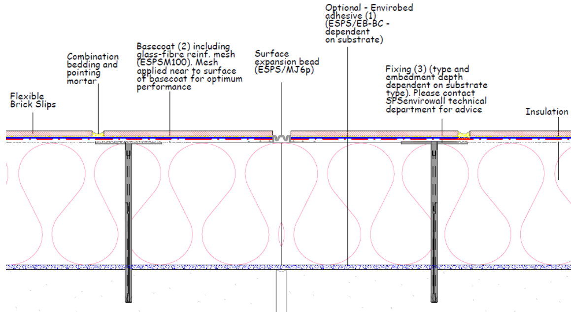
Diagram 5 - Surface expansion bead
